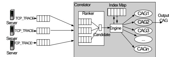
Fig.2. The architecture of PreciseTracer
